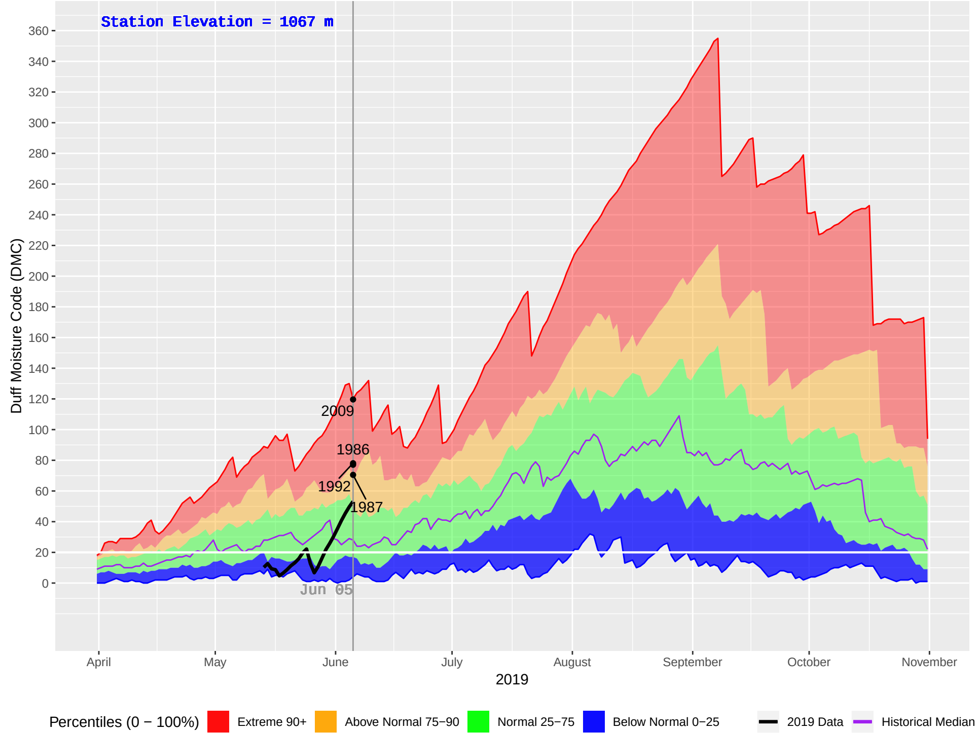
MCCUDDY (334) : Historical (1984–2018), Current (2019) Daily Duff Moisture Code (DMC)
