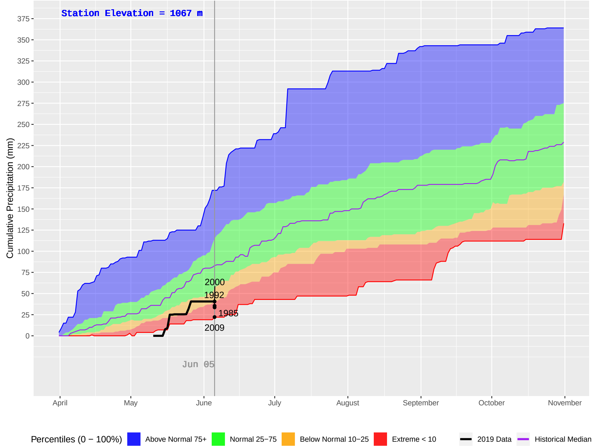
MCCUDDY (334) : Historical (1984–2018), Current (2019) Daily Cumulative Precipitation
