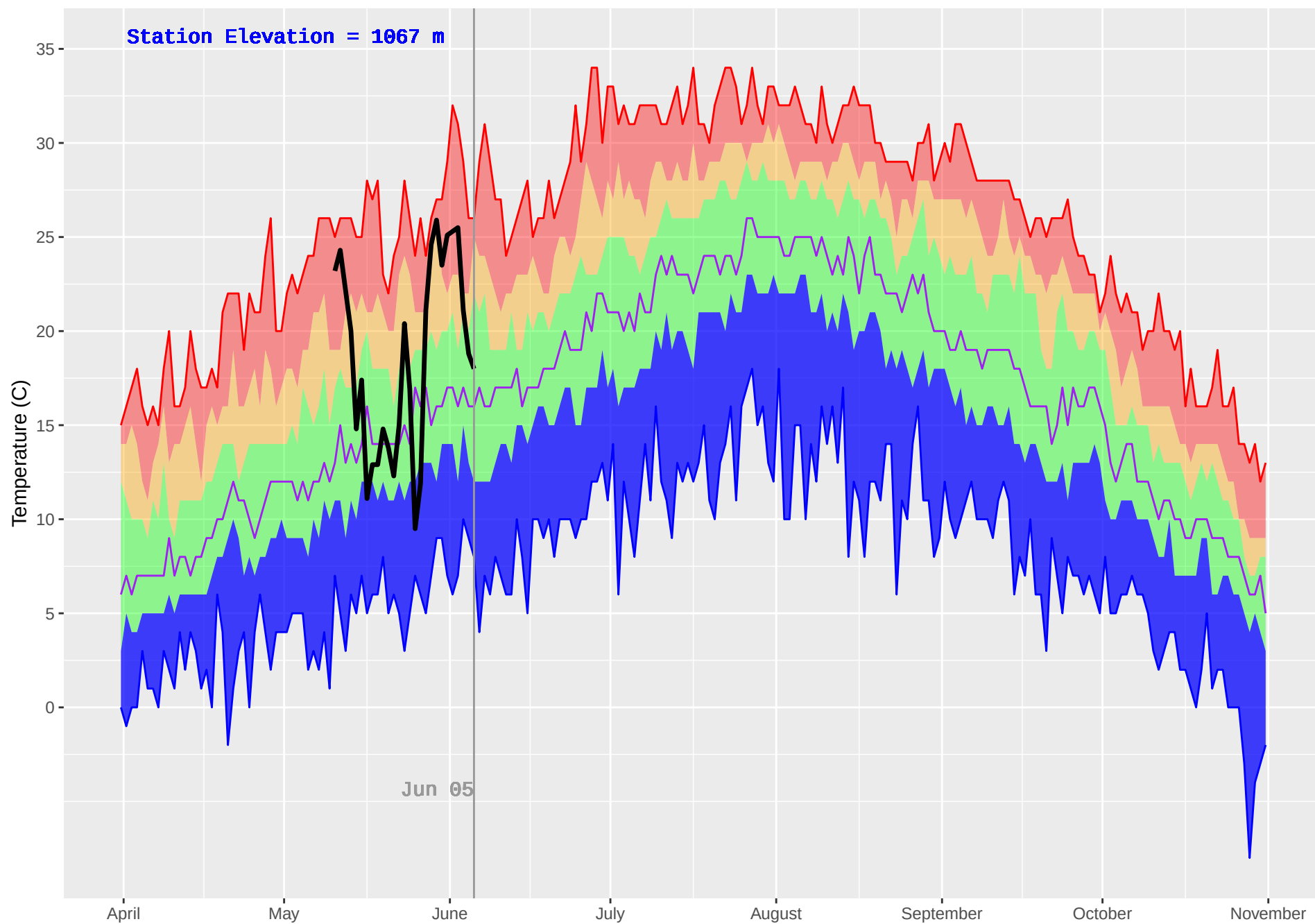
MCCUDDY (334) : Historical (1984–2018) and Current (2019) Daily Temperature
