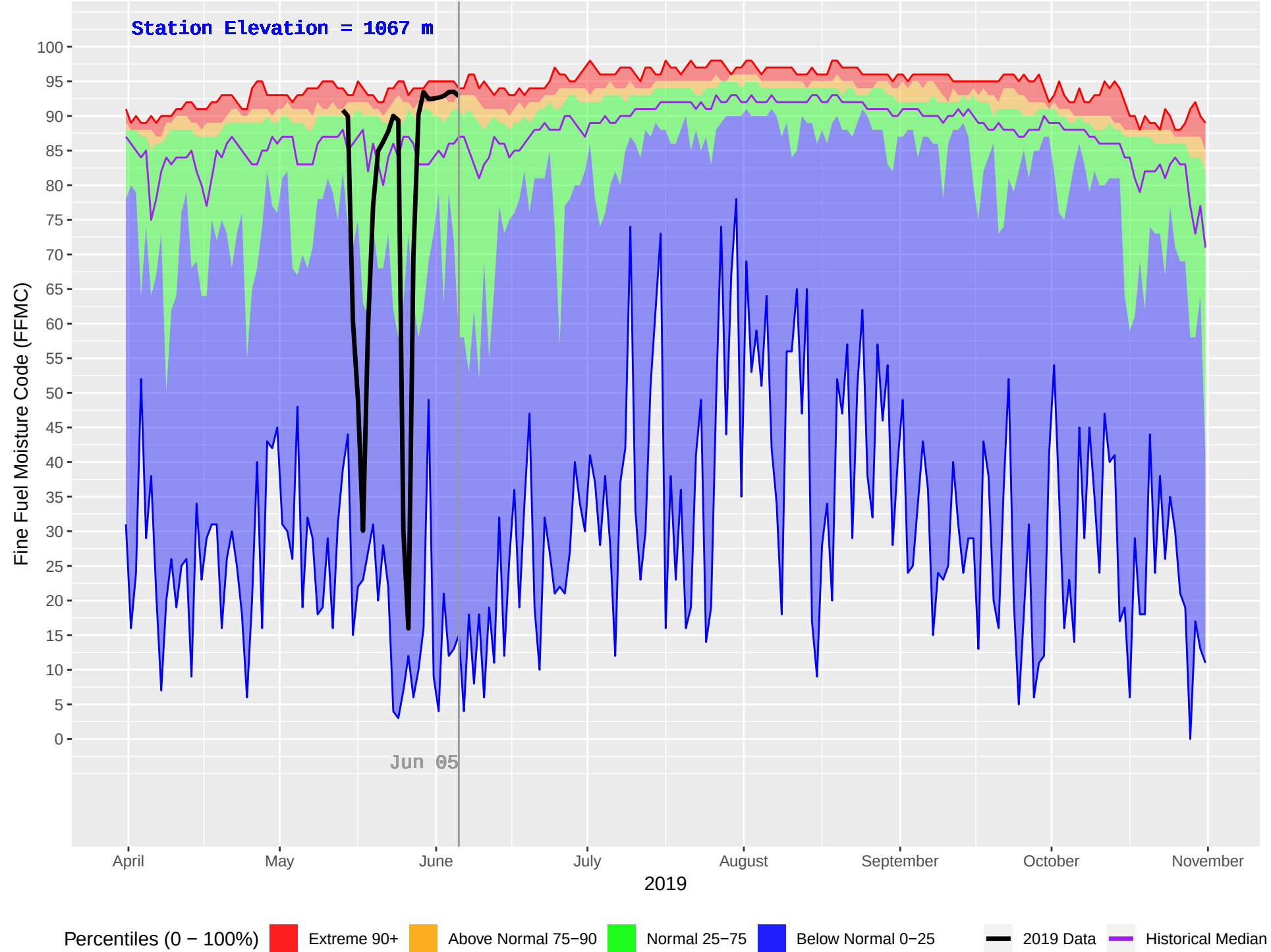
MCCUDDY (334) : Historical (1984–2018) and Current (2019) Daily Fine Fuel Moisture Code (FFMC)
