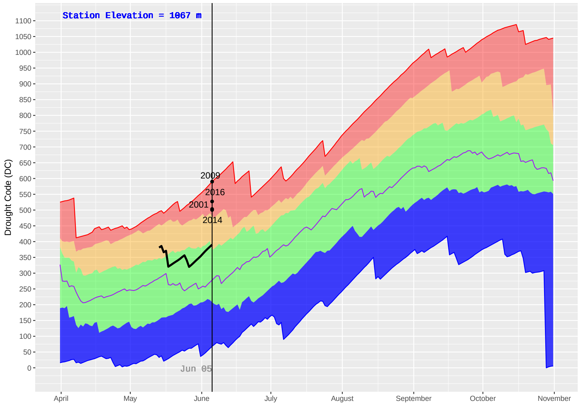
MCCUDDY (334) : Historical (1984–2018) and Current (2019) Daily Drought Code (DC)
