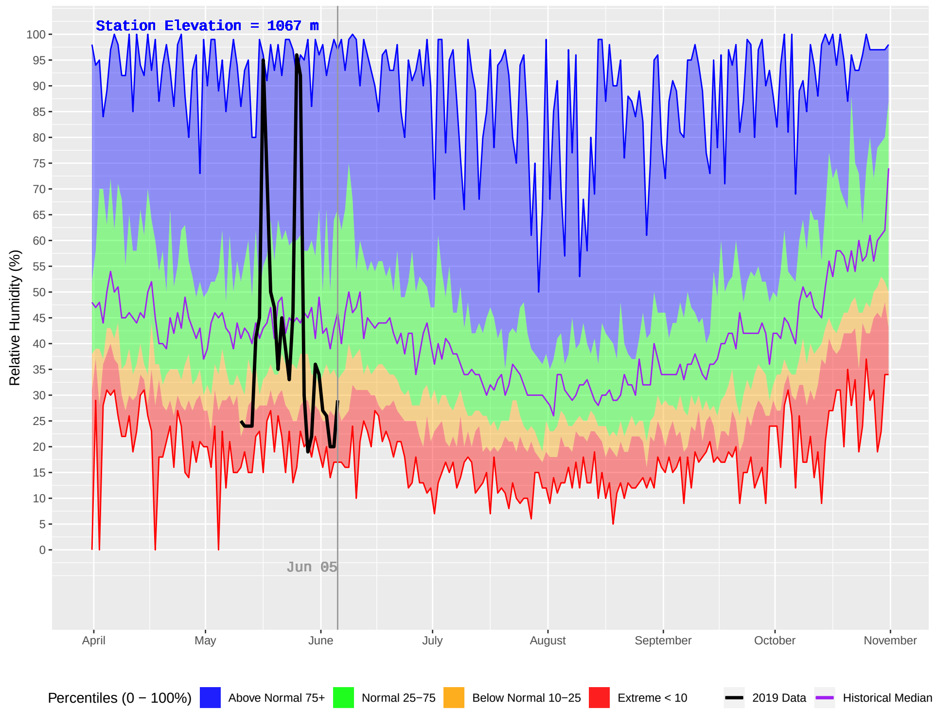
MCCUDDY (334) : Historical (1984–2018) and Current (2019) Daily Relative Humidity
